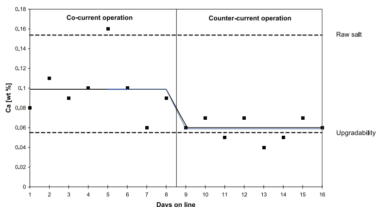
Fig 4: Co-current vs. counter-current process performance
