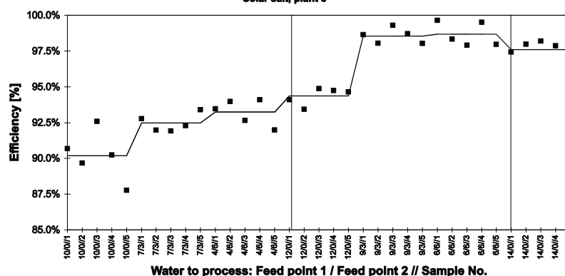
Fig 5: SALEX-B optimisation test: NaCl efficiencies
